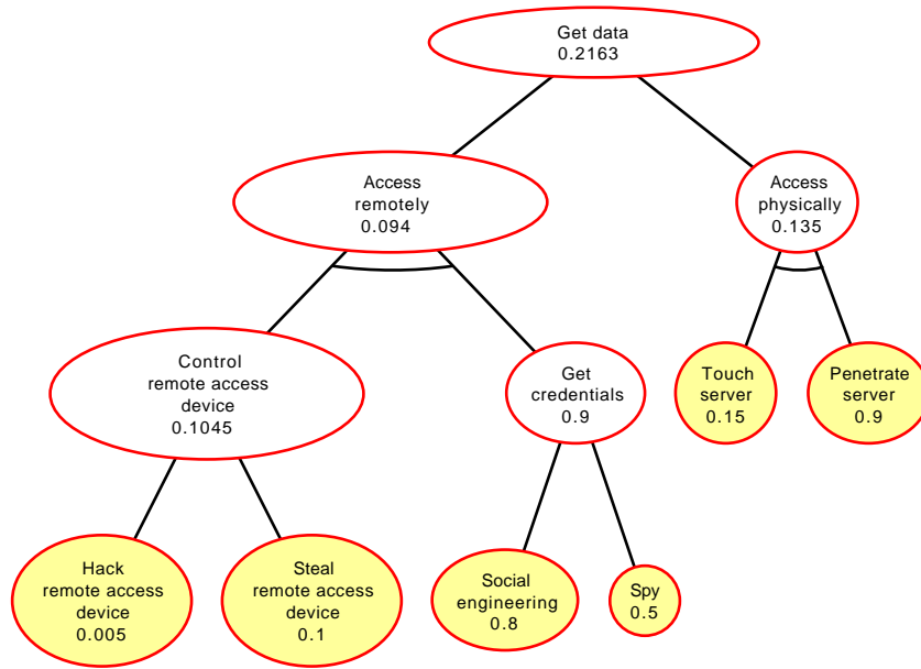
Fig. 1. Initial attack tree with success probabilities for our private cloud attack use case.
